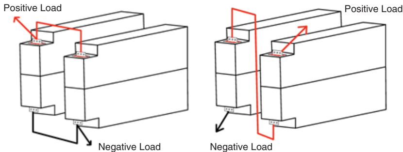
Parallel Connection, 12V 540Ah bank Increases Ah, Voltage stays the same.
