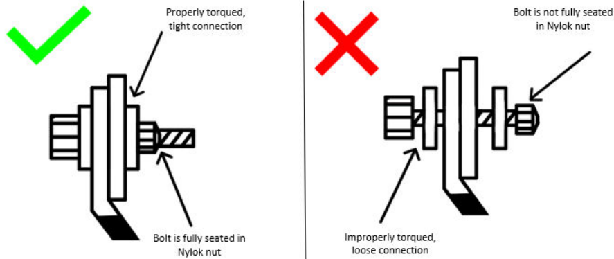
Figure 2: Proper and Improper Terminal Connections
