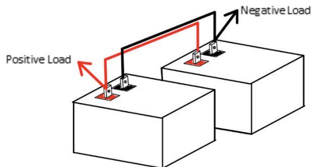
Figure 3: Two 8D Batteries connected in Parallel to create a 12V 540Ah Battery Bank
