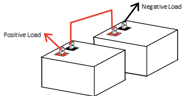
Figure 4: Two 8D Batteries Connected in Series to create a 24V 270Ah Battery Bank
