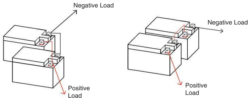
Parallel Connection, 24V 100Ah bank Increases Ah, Voltage stays the same.
